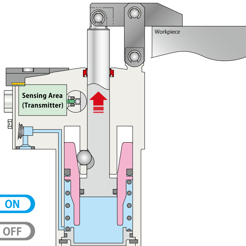
Clamped State
